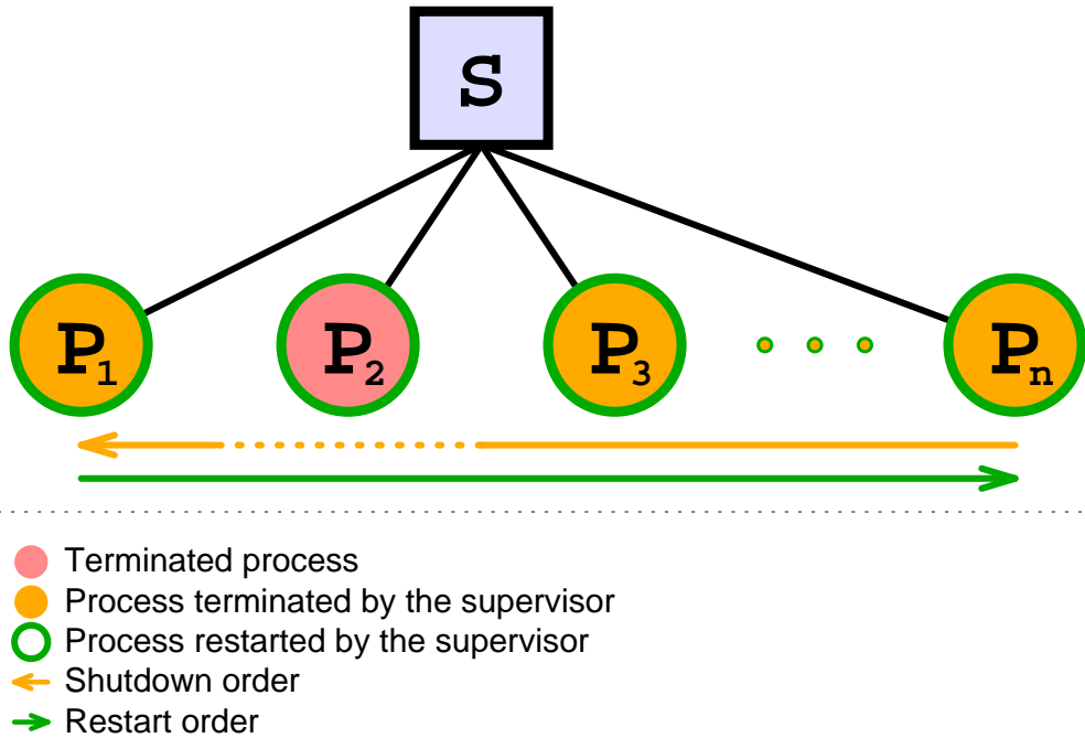
Figure 5.2: One_For_All Supervision
